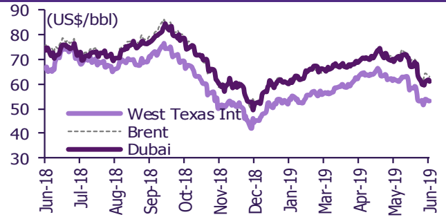
Crude prices
