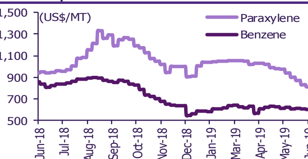
Aromatics prices
