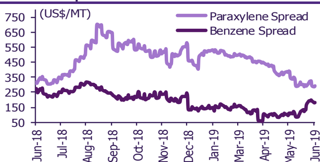
Aromatics spreads
